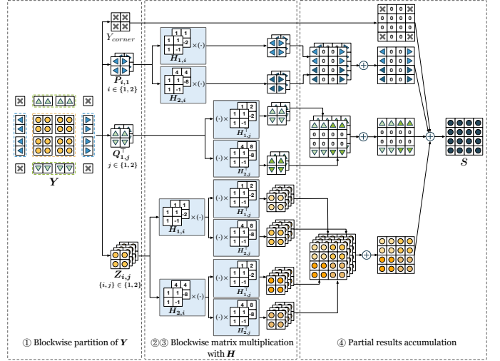
Figure 6: Blockwise Output Transformation for F(4, 3) . The ①②③④ correspond to ❶❷❸❹ of BOT procedure in Section 3.3.
